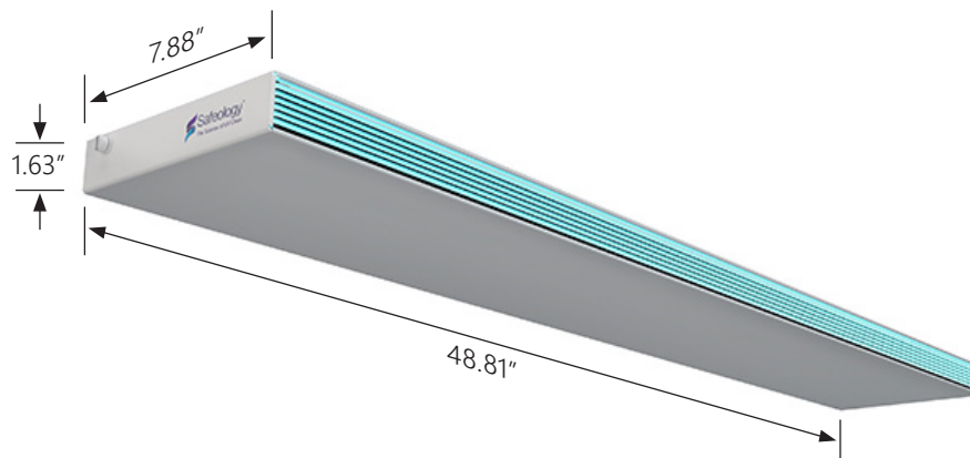
SERIES R UVC Upper Room Linear Wall Fixture Model SRLW
